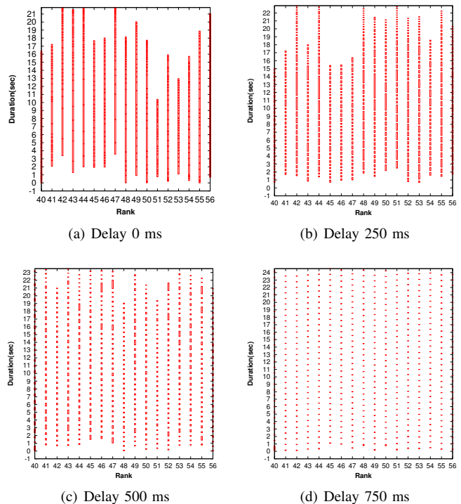
Fig. 16: Timelines per process with delays between each I/O request.
